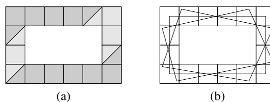
Figure 5: Discrete segment recognition and reconstruction. (a) Recognized discrete segments. Bicolor pixels belong to two discrete segments. (b) Three possible reconstructions for a same discrete curve.
