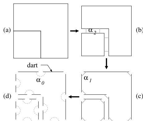
Figure 1: Topological decomposition of an object. (a) A 2D Euclidean object. (b) Its decomposition into topological faces. (c) Faces decomposition into topological edges. (d) Edges decomposition into darts.
