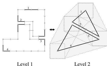
Figure 12: Links between level 1 and level 2. Black darts are connected ones. For example, darts numbered 1 (resp. 2, 3 and 4) in the two representations are together connected. Here, there are exactly 12 links between the two levels.
