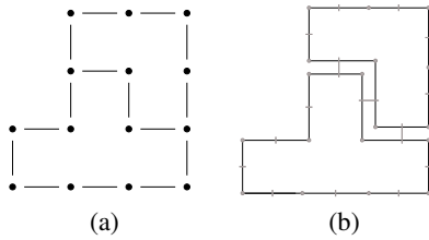
Figure 8: The discrete border level. (a) Discrete border view. (b) Discrete border 2-G-map.
