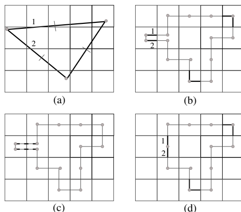
Figure 13: Example of degenerated vertex. (a) Level 2 primitive. (b) Primitive computed according to the standard discretization process. (c) Dashed darts are removed. (d) Level 1 primitive obtained. Note that black darts are connected ones.
