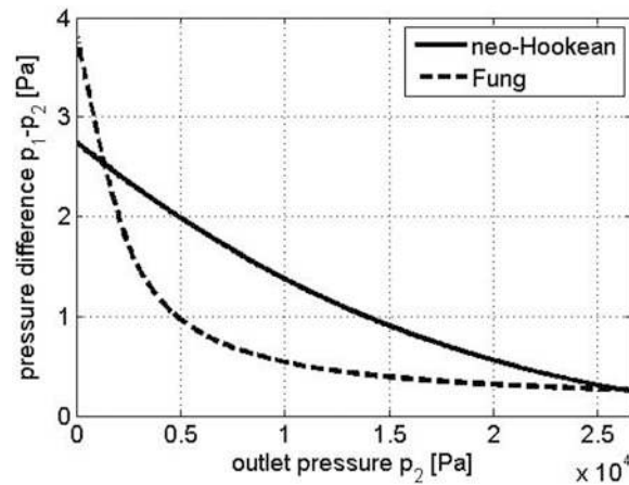
Fig. 6. Dependence of the difference between the inlet and outlet pressure on the outlet pressure with constant inner flow Q = 2 \text{ ml/min}
